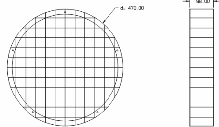
Protection grid 111287
