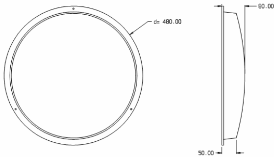
Polycarbonate-protection 111286
